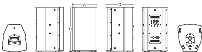
Dimension(W×H×D):245×447×320mm
